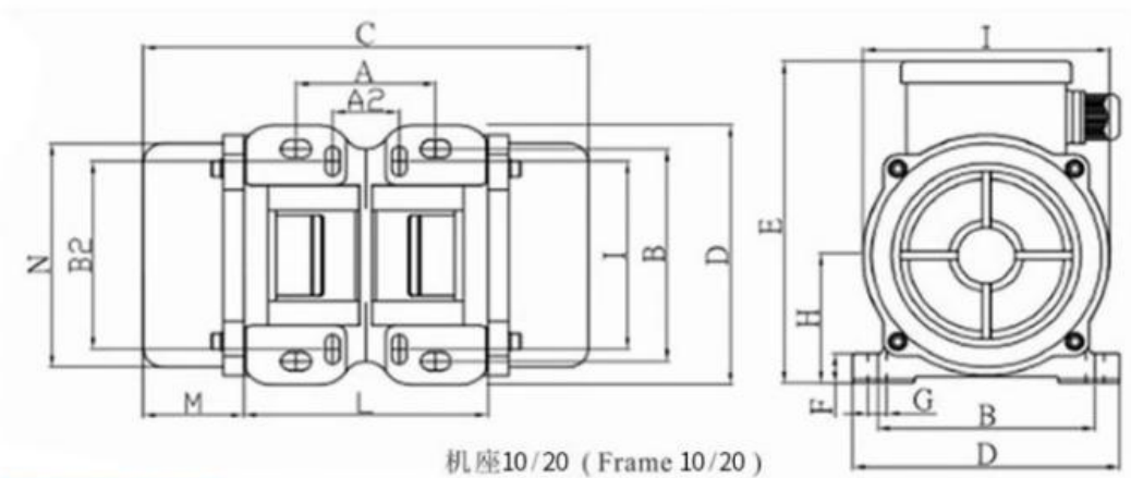
安装外形尺寸表 Installation of overall dimension 单位Unit: mm
