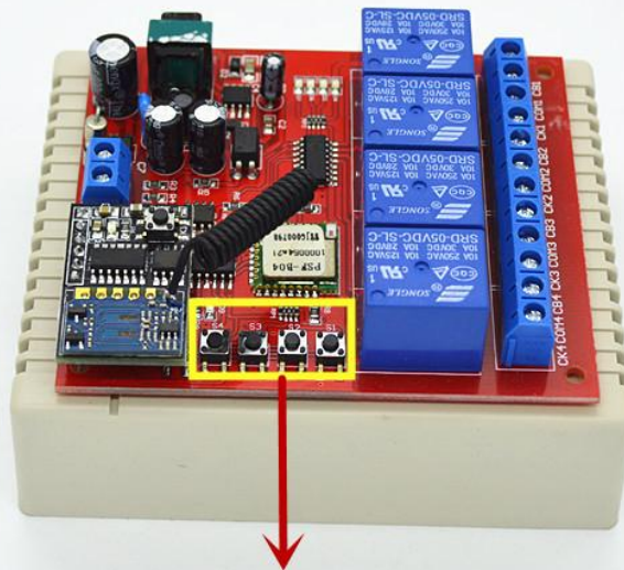
Manual control button
